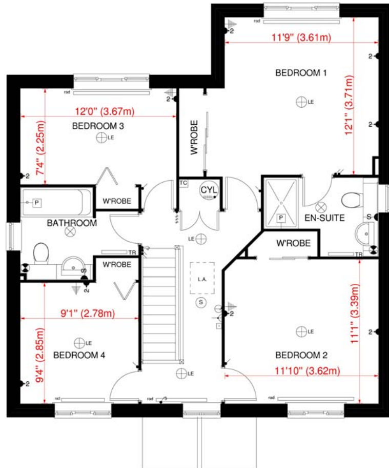
FIRST FLOOR PLAN (Handed) 'WILBERFORCE' HOUSE TYPE - PLOT 1, SPROWSTON
