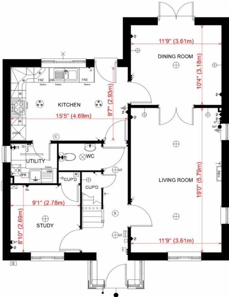
GROUND FLOOR PLAN (Handed) 'WILBERFORCE' HOUSE TYPE - PLOT 1, SPROWSTON
