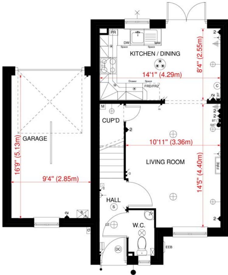
GROUND FLOOR PLAN (Handed) VAUGHAN 'E' HOUSE TYPE - SPROWSTON
