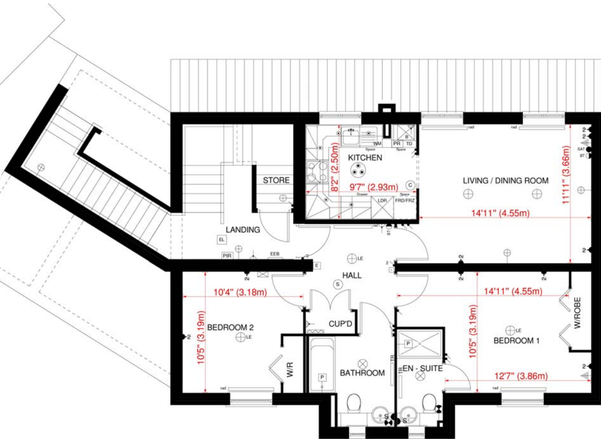
FIRST FLOOR PLAN 'RUSKIN' HOUSE TYPE - PLOT 51, SPROWSTON.
