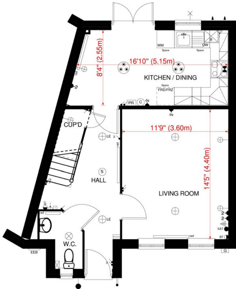
GROUND FLOOR PLAN (Handed) 'JOHNSON 'A' HOUSE TYPE - SPROWSTON
