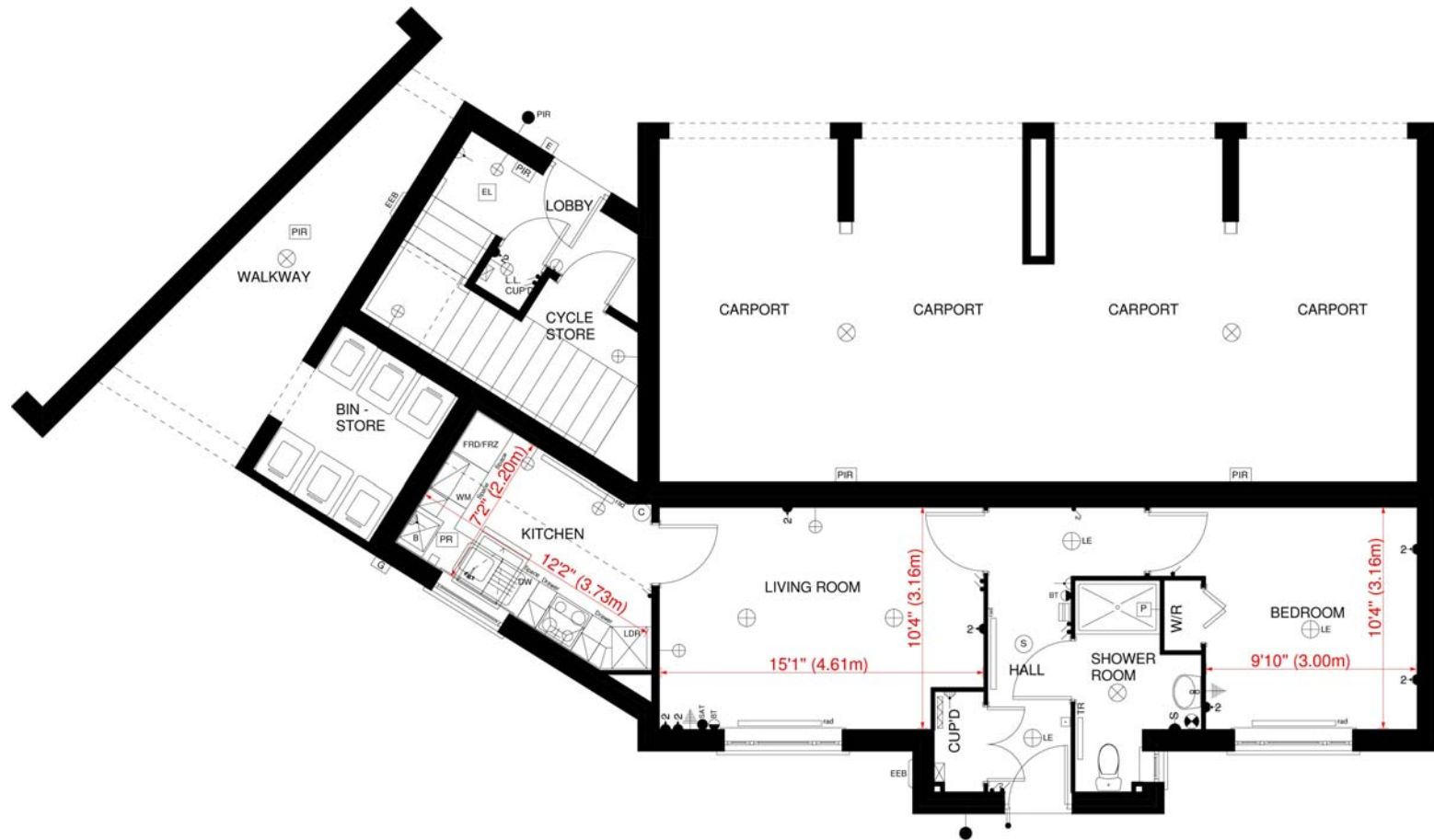
GROUND FLOOR PLAN 'HUXLEY' HOUSE TYPE - PLOTS 45 & 50, SPROWSTON.
