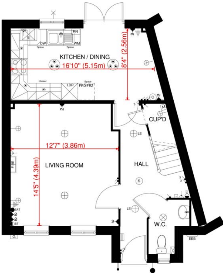
GROUND FLOOR PLAN CARTWRIGHT 'A' HOUSE TYPE - SPROWSTON
