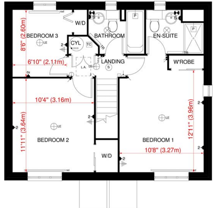
FIRST FLOOR PLAN 'BYRON' HOUSE TYPE - SPROWSTON
