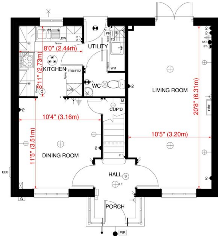
GROUND FLOOR PLAN 'BYRON' HOUSE TYPE - SPROWSTON
