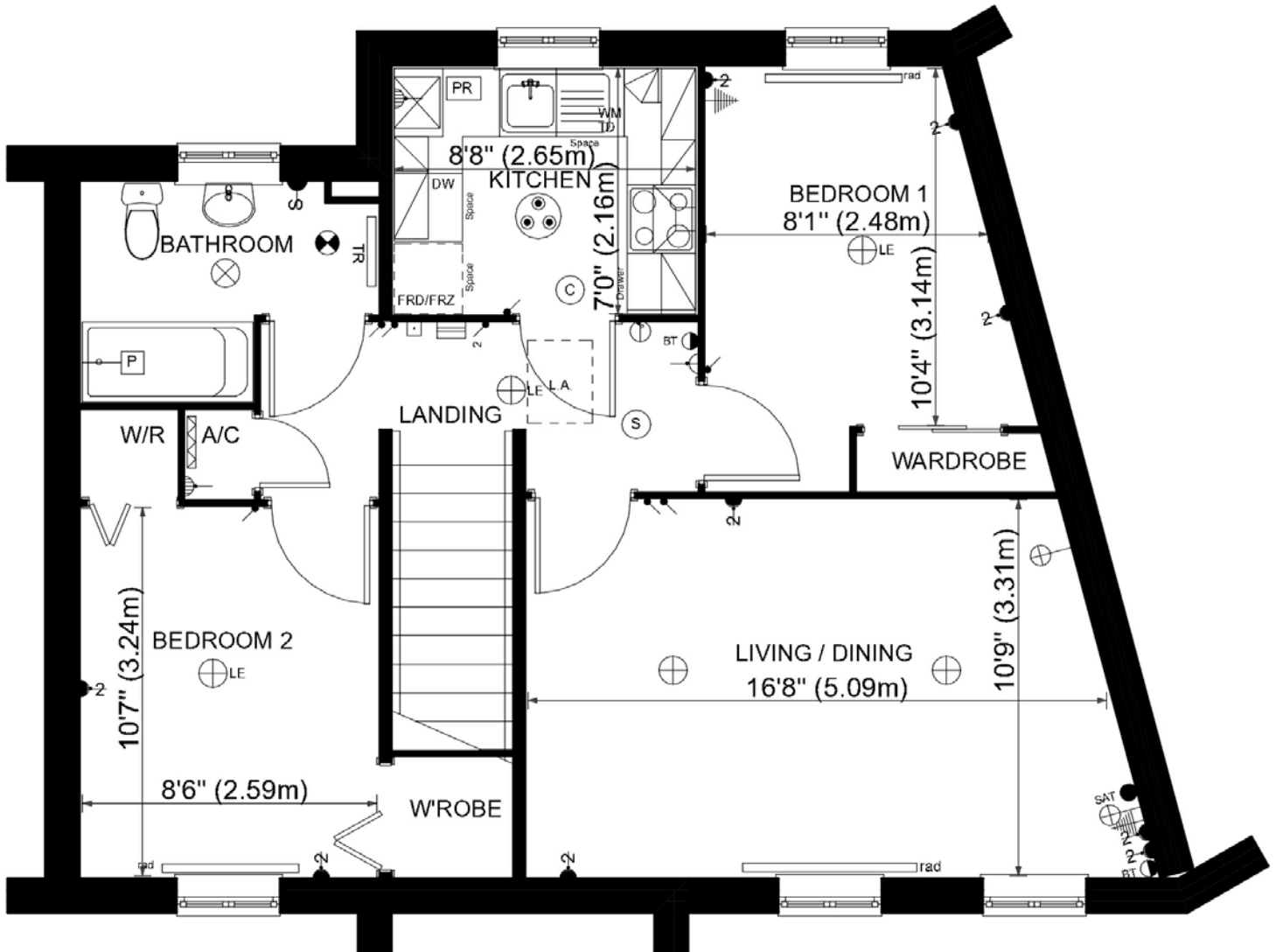
FIRST FLOOR PLAN 'BRUNEL' HOUSE TYPE - PLOTS 4 & 6, SPROWSTON.
