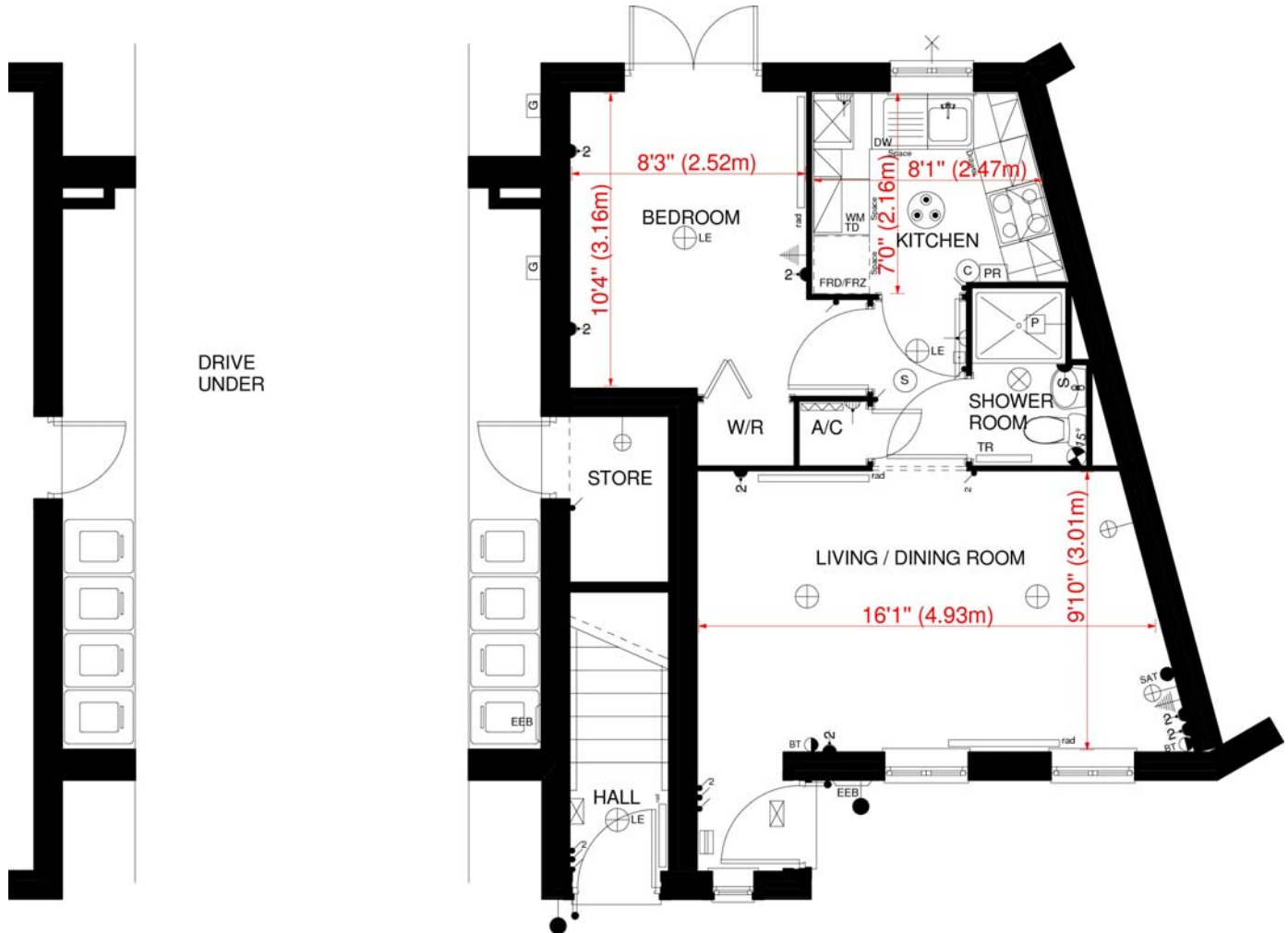
GROUND FLOOR PLAN 'BAIRD' HOUSE TYPE - PLOTS 3 & 5, SPROWSTON.
