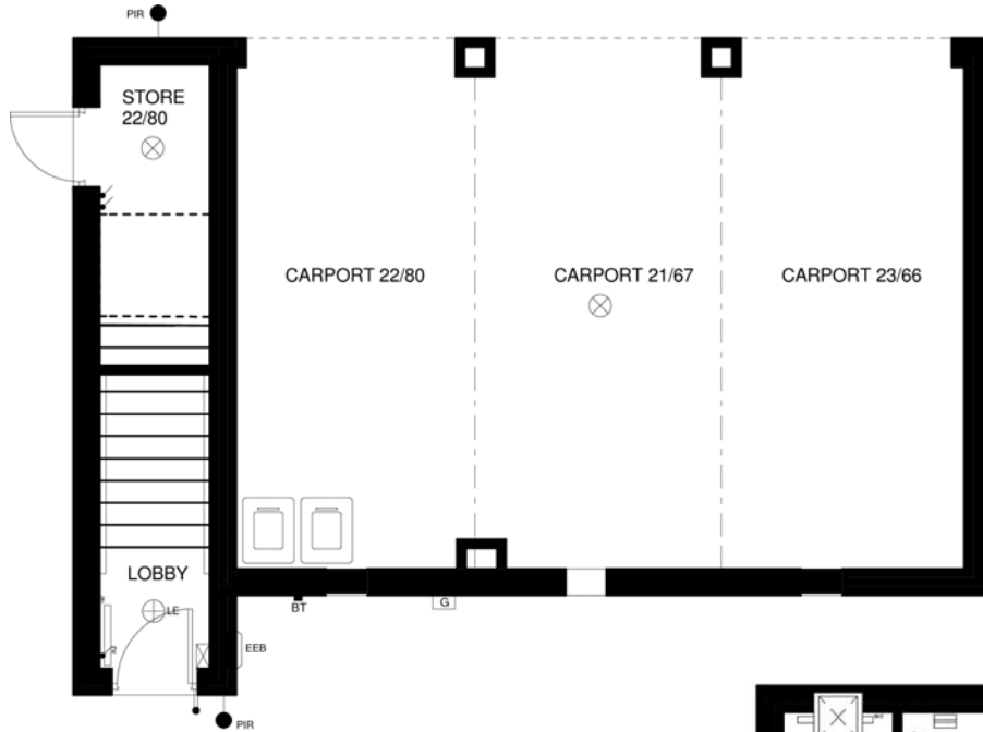
GROUND FLOOR PLAN 'BABBAGE' HOUSE TYPE - PLOTS 22 & 80, SPROWSTON
