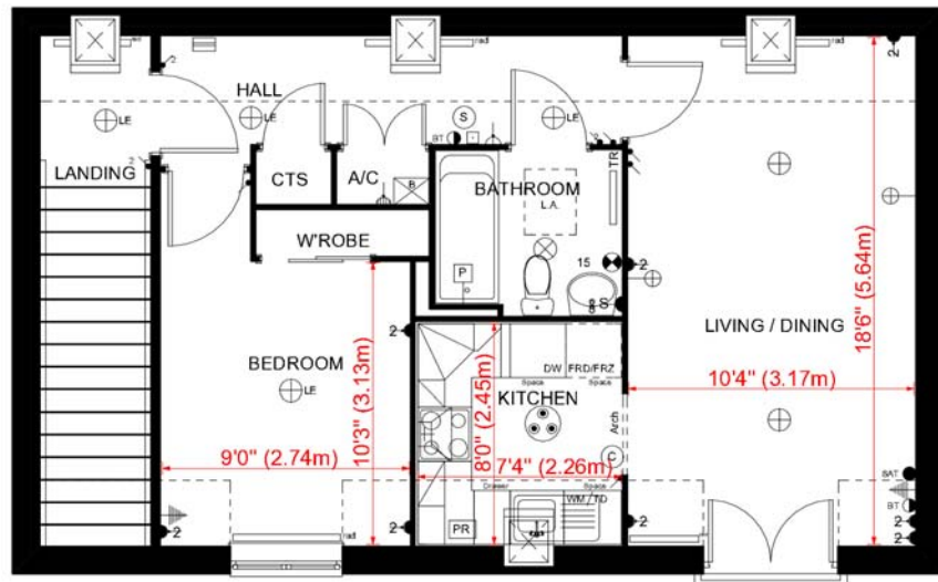
GROUND FLOOR PLAN 'BABBAGE' HOUSE TYPE - PLOTS 22 & 80, SPROWSTON
