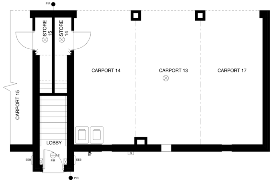
GROUND FLOOR PLAN 'BABBAGE 'A' HOUSE TYPE - SPROWSTON
