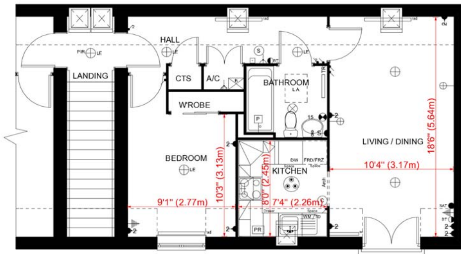
GROUND FLOOR PLAN 'BABBAGE 'A' HOUSE TYPE - SPROWSTON
