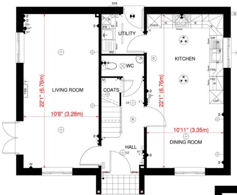
GROUND FLOOR PLAN 'ADDINGTON 'A' HOUSE TYPE - SPROWSTON
