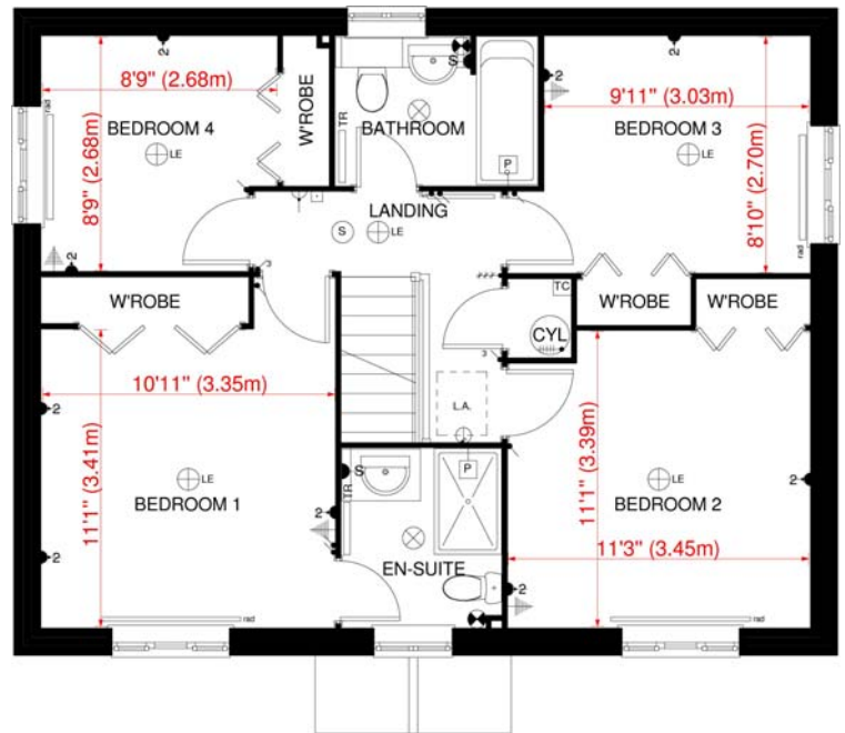
FIRST FLOOR PLAN 'ADDINGTON 'A' HOUSE TYPE - SPROWSTON
