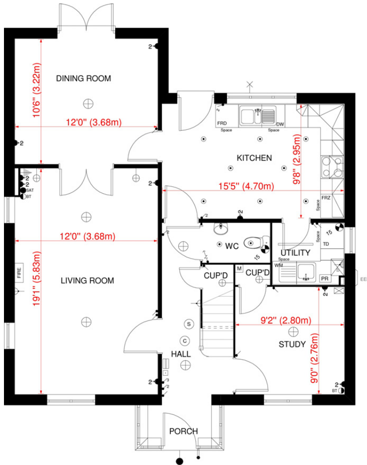
GROUND FLOOR PLAN 'WILBERFORCE' HOUSE TYPE - HEMSBY
