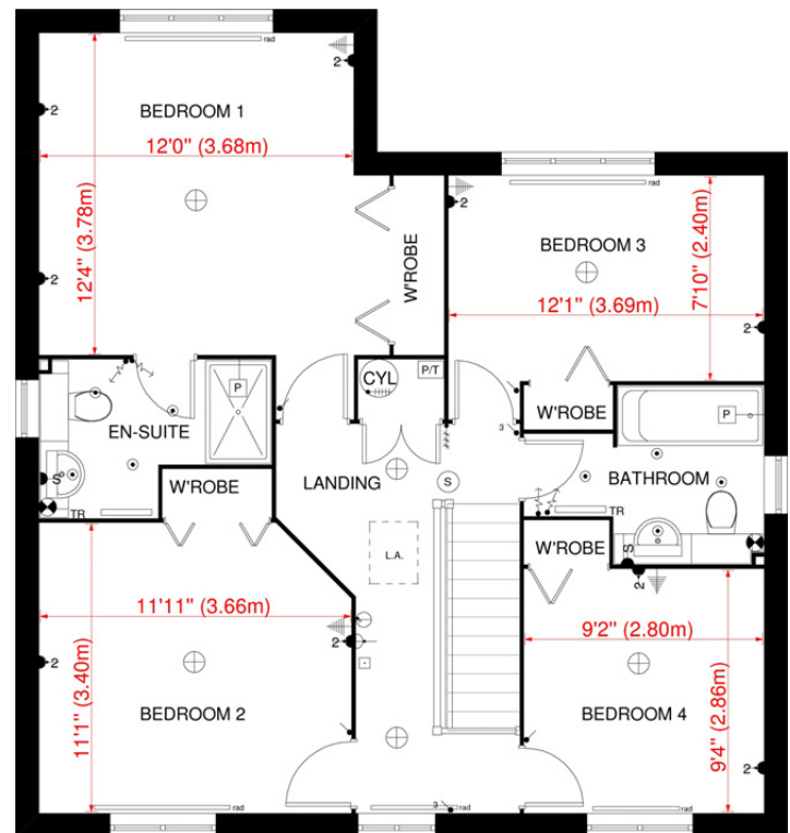
FIRST FLOOR PLAN 'WILBERFORCE' HOUSE TYPE - HEMSBY
