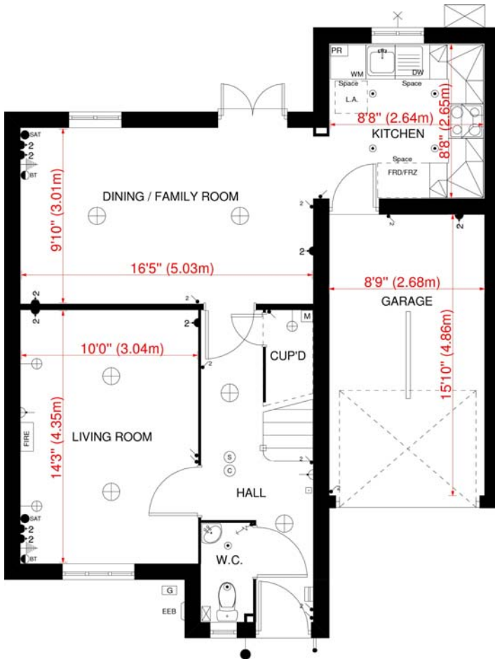
GROUND FLOOR PLAN 'VAUGHAN 'D' HOUSE TYPE - HEMSBY
