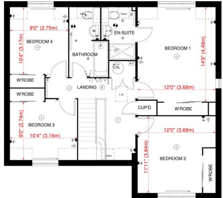
FIRST FLOOR PLAN 'NIGHTINGALE' HOUSE TYPE - HEMSBY
