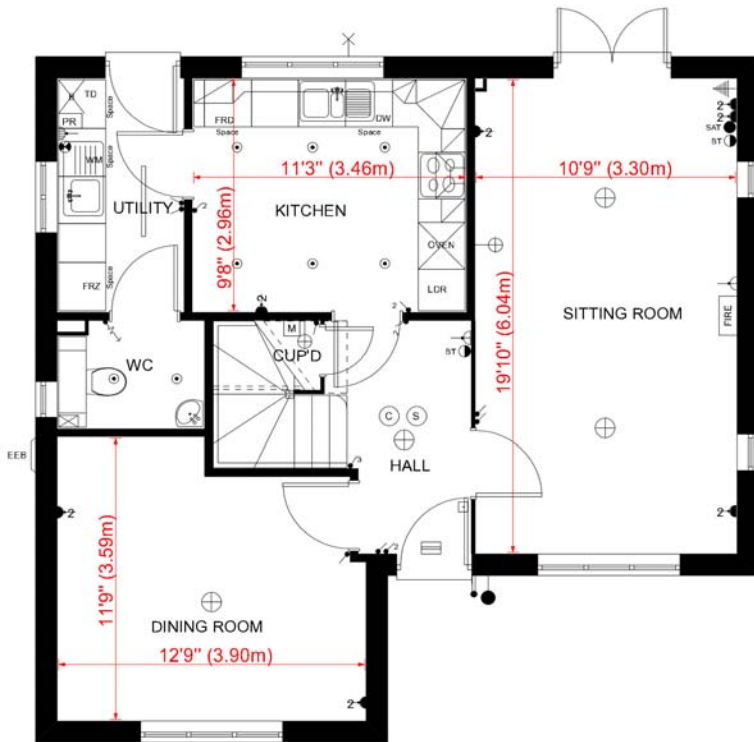
GROUND FLOOR PLAN 'MOUNTBATTEN' HOUSE TYPE - PLOT 77 Only, HEMSBY
