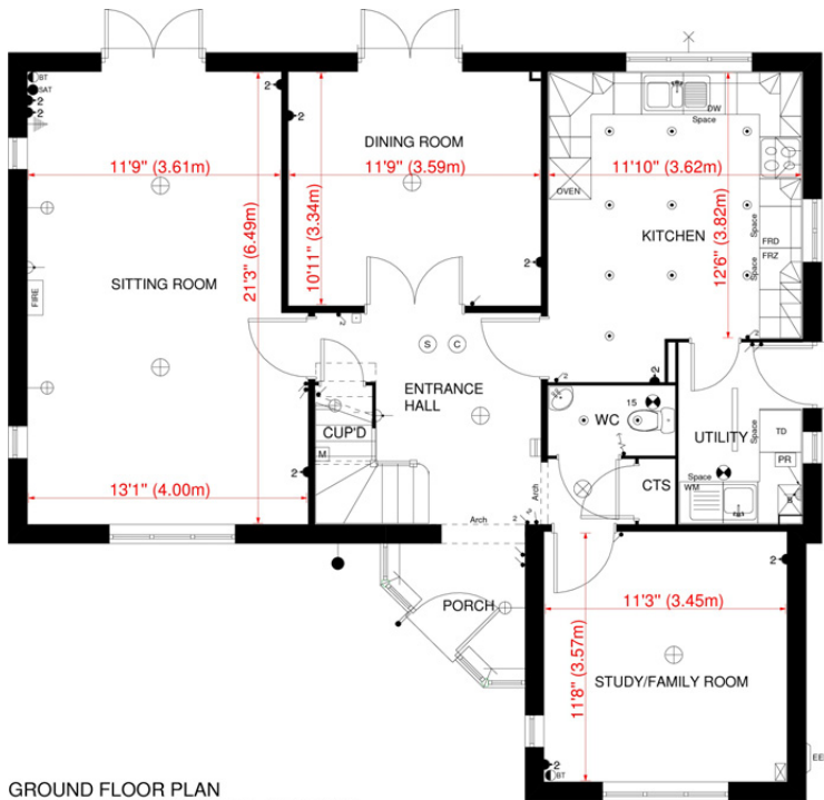
GROUND FLOOR PLAN 'FROBISHER' HOUSE TYPE - HEMSBY
