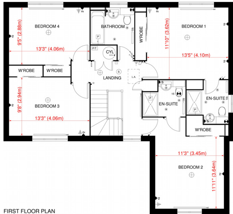
FIRST FLOOR PLAN 'FROBISHER' HOUSE TYPE - HEMSBY
