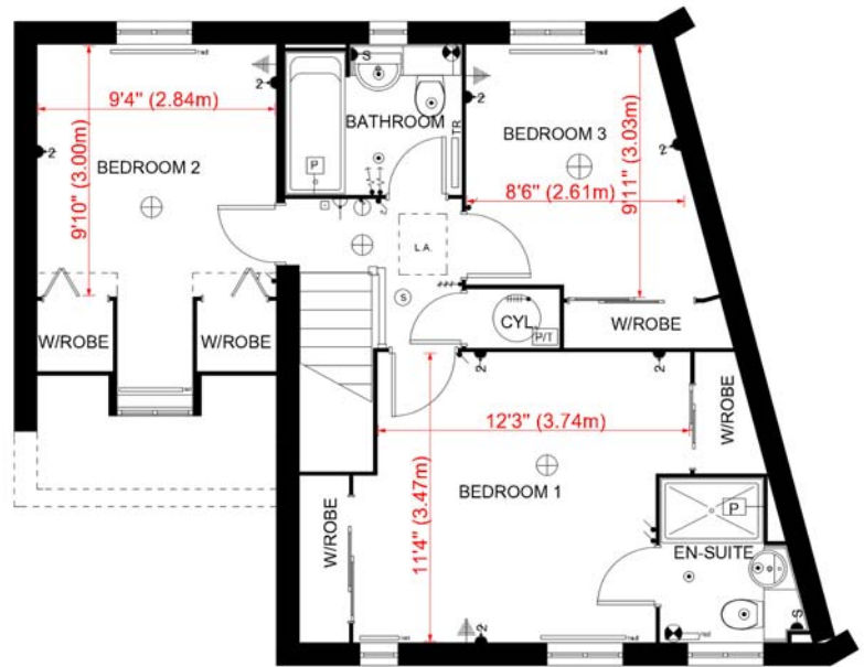
FIRST FLOOR PLAN 'COLERIDGE B' HOUSE TYPE - HEMSBY.
