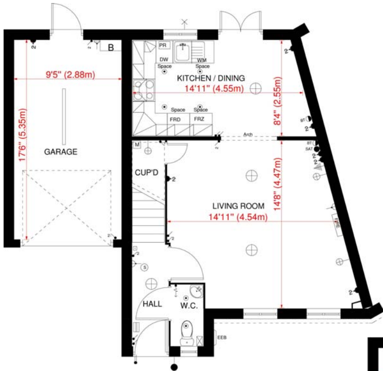
GROUND FLOOR PLAN 'COLERIDGE B' HOUSE TYPE - HEMSBY.
