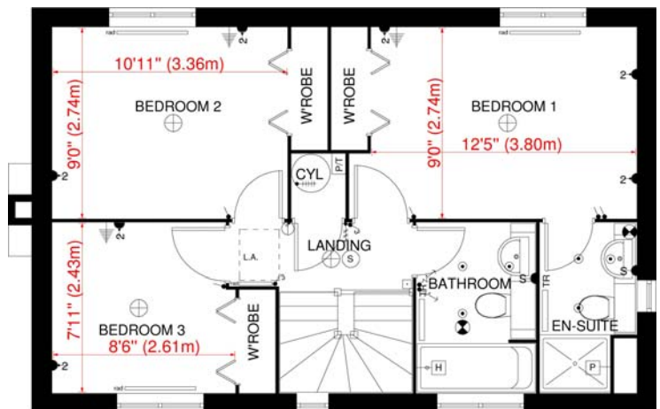
'BINGHAM' HOUSE TYPE - HEMSBY FIRST FLOOR PLAN
