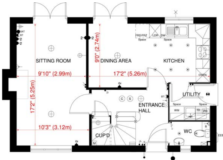
'BINGHAM' HOUSE TYPE - HEMSBY GROUND FLOOR PLAN
