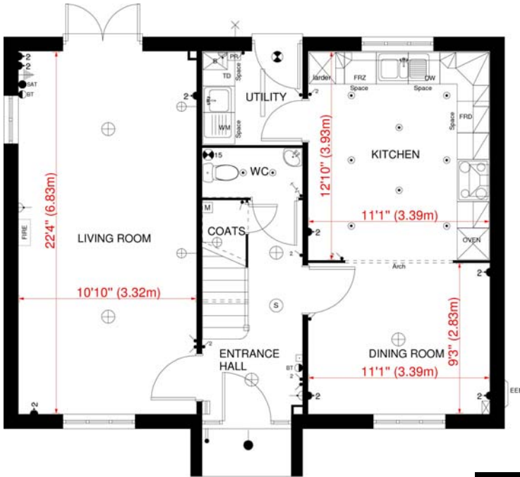
GROUND FLOOR PLAN 'ADDINGTON 'H' HOUSE TYPE - HEMSBY
