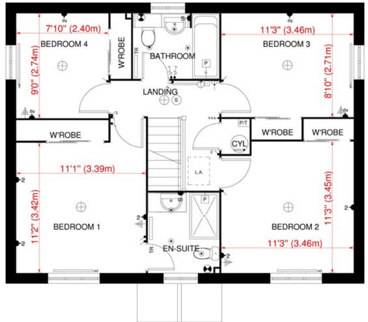
FIRST FLOOR PLAN 'ADDINGTON 'H' HOUSE TYPE - HEMSBY
