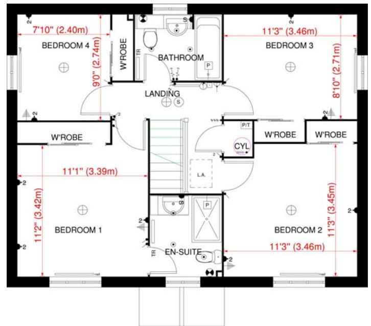
FIRST FLOOR PLAN 'ADDINGTON D' HOUSE TYPE - HEMSBY
