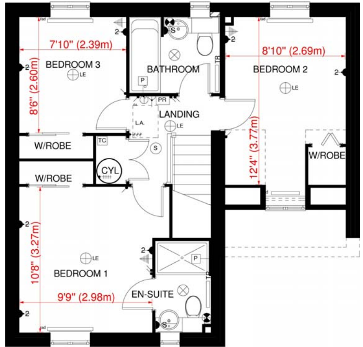
FIRST FLOOR PLAN 'VAUGHAN' HOUSE TYPE - SOUTH GREEN
