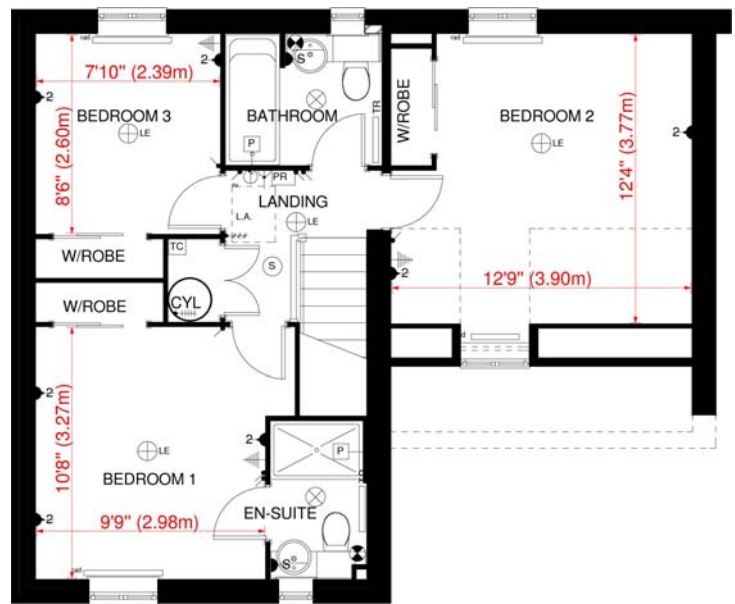
FIRST FLOOR PLAN VAUGHAN 'B' HOUSE TYPE - SOUTH GREEN
