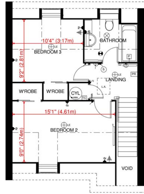
SECOND FLOOR PLAN 'LANDSEER 'A' HOUSE TYPE - SOUTH GREEN
