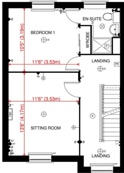
FIRST FLOOR PLAN 'LANDSEER 'A' HOUSE TYPE - SOUTH GREEN
