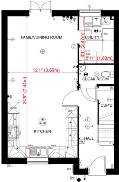
GROUND FLOOR PLAN 'LANDSEER 'A' HOUSE TYPE - SOUTH GREEN
