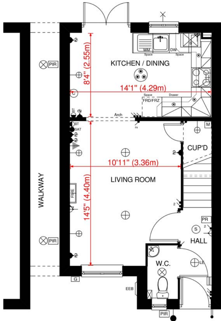
GROUND FLOOR PLAN 'ASTON' HOUSE TYPE - SOUTH GREEN
