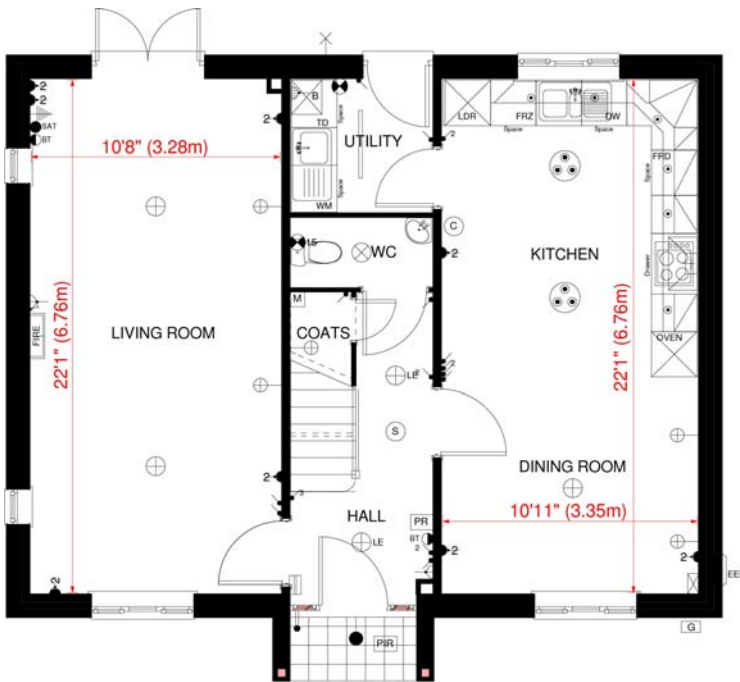
GROUND FLOOR PLAN 'ADDINGTON' HOUSE TYPE - SOUTH GREEN
