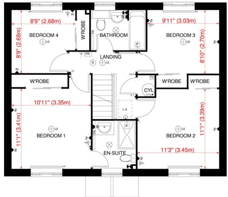
FIRST FLOOR PLAN 'ADDINGTON' HOUSE TYPE - SOUTH GREEN
