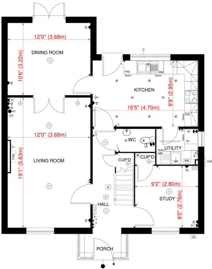
GROUND FLOOR PLAN 'WILBERFORCE' HOUSE TYPE - BRADWELL
