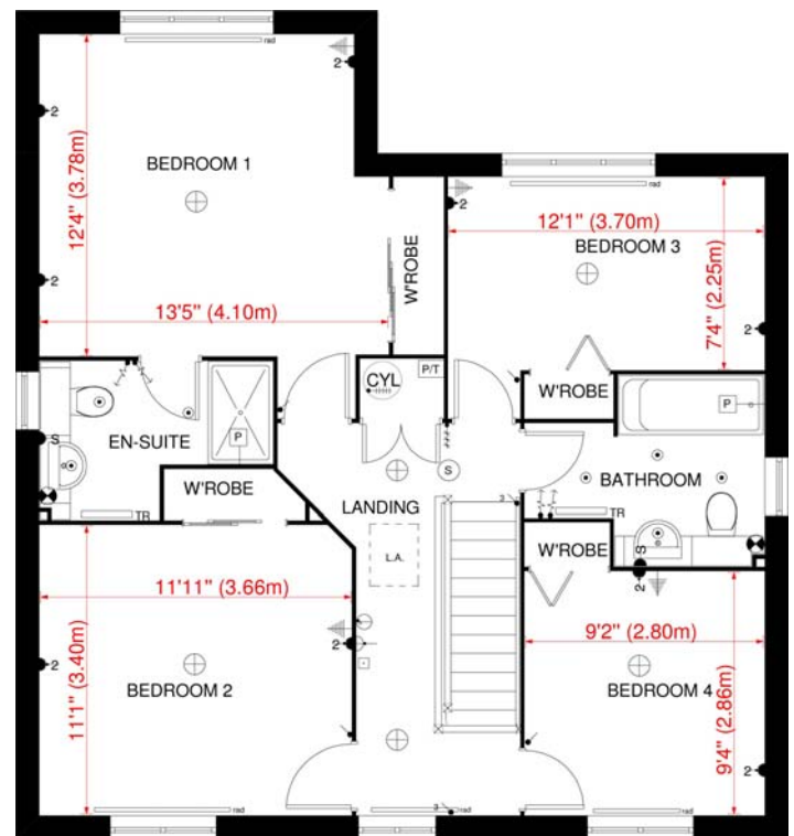
FIRST FLOOR PLAN 'WILBERFORCE' HOUSE TYPE - BRADWELL
