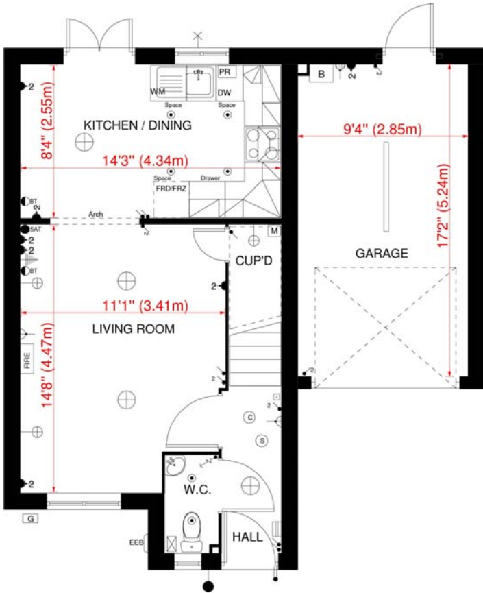
GROUND FLOOR PLAN 'VAUGHAN' HOUSE TYPE - BRADWELL
