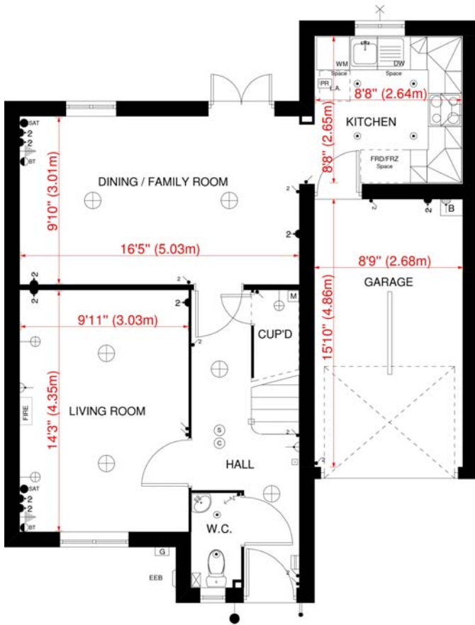
GROUND FLOOR PLAN 'VAUGHAN 'D' HOUSE TYPE - BRADWELL
