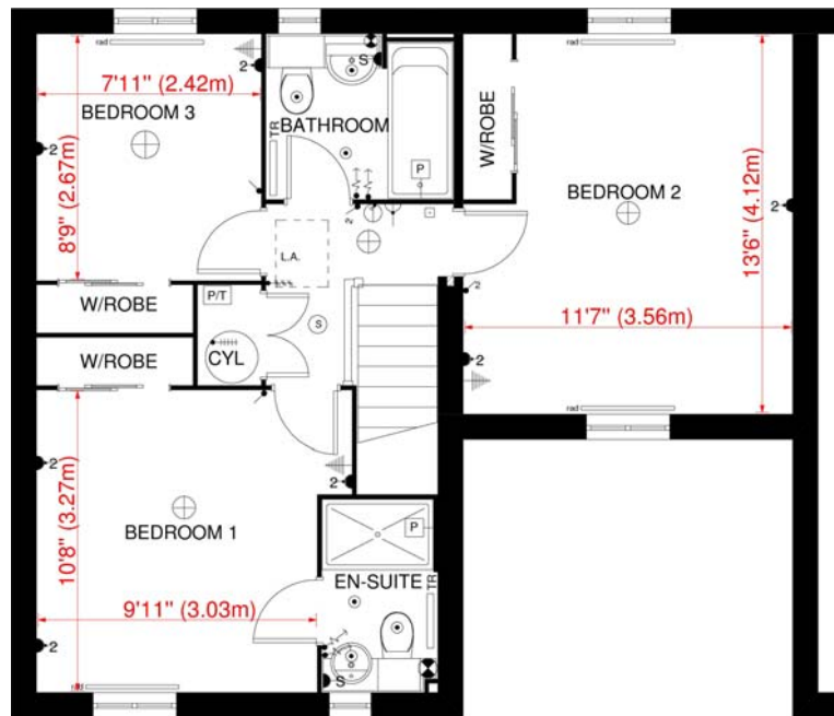
FIRST FLOOR PLAN VAUGHAN 'C' HOUSE TYPE - BRADWELL
