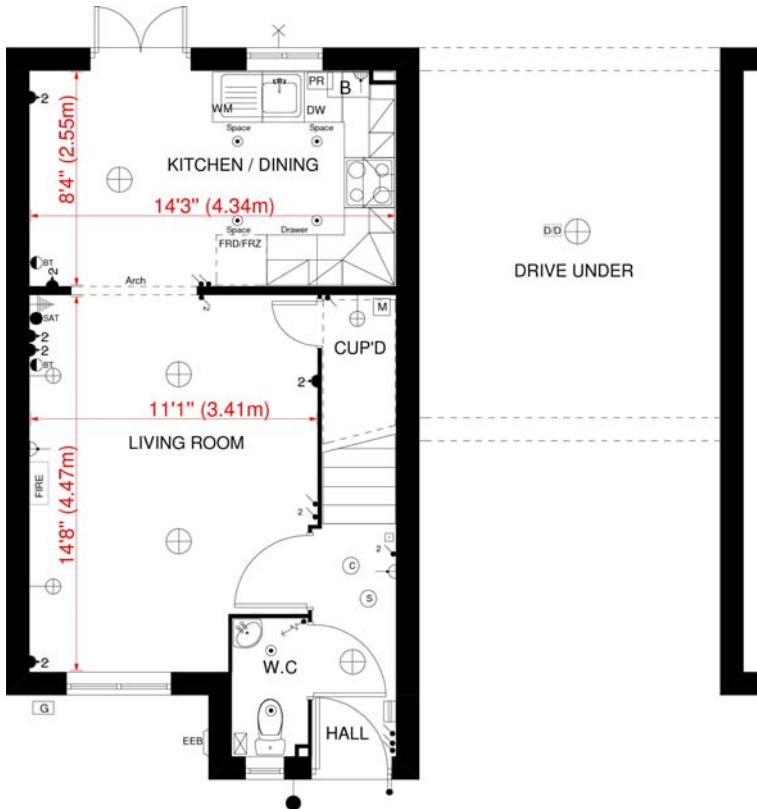
GROUND FLOOR PLAN VAUGHAN 'C' HOUSE TYPE - BRADWELL.
