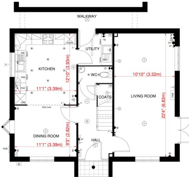
GROUND FLOOR PLAN FARADAY HOUSE TYPE - BRADWELL
