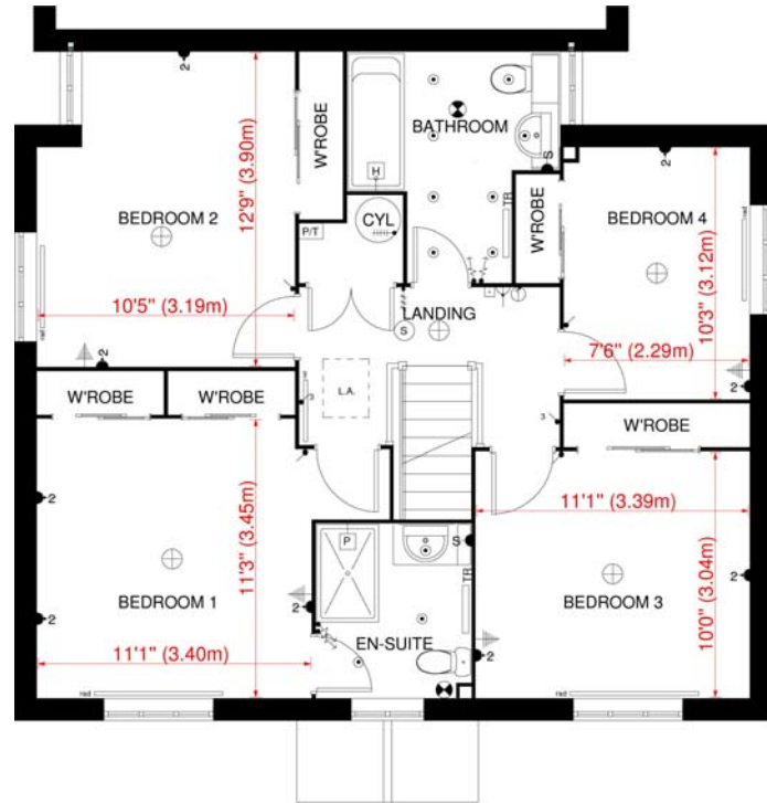
FIRST FLOOR PLAN FARADAY HOUSE TYPE - BRADWELL
