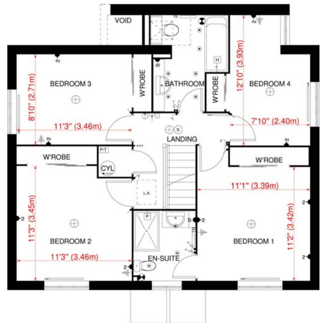
FIRST FLOOR PLAN FARADAY 'A' HOUSE TYPE - BRADWELL
