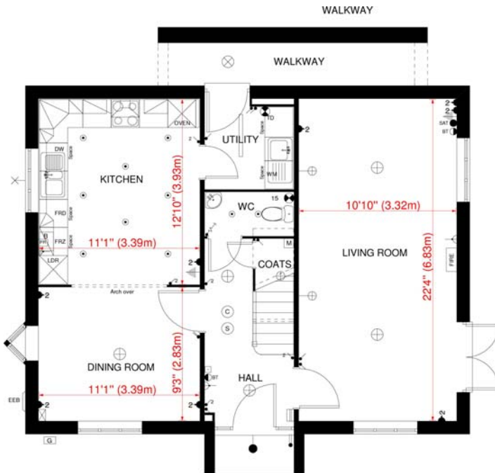
GROUND FLOOR PLAN FARADAY 'A' HOUSE TYPE - BRADWELL
