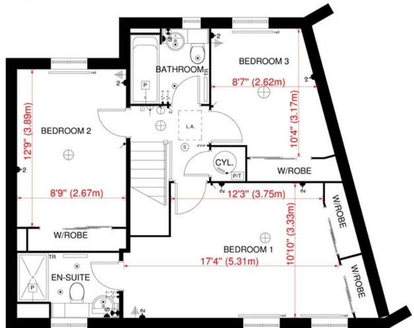
FIRST FLOOR PLAN 'BLAKE' HOUSE TYPE - BRADWELL
