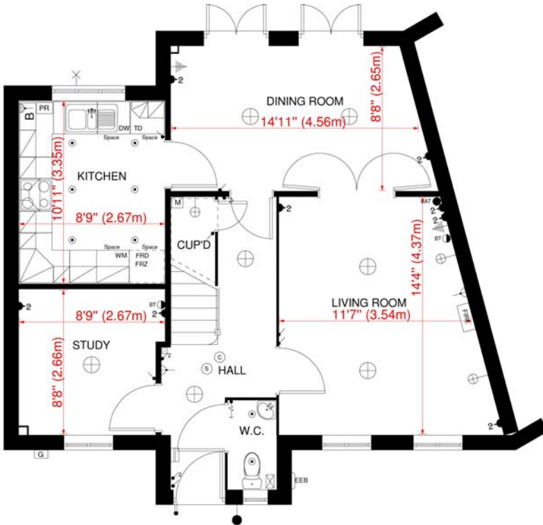
GROUND FLOOR PLAN 'BLAKE' HOUSE TYPE - BRADWELL
