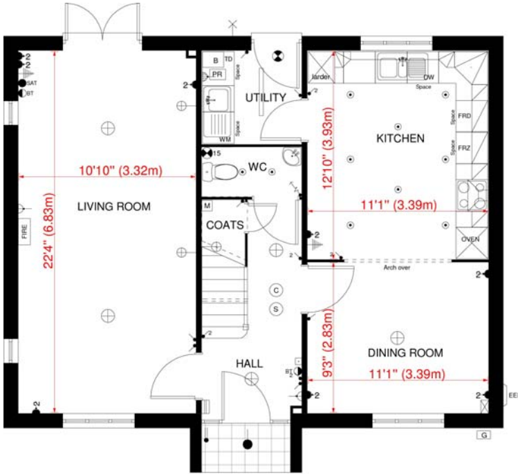
GROUND FLOOR PLAN 'ADDINGTON' HOUSE TYPE - BRADWELL
