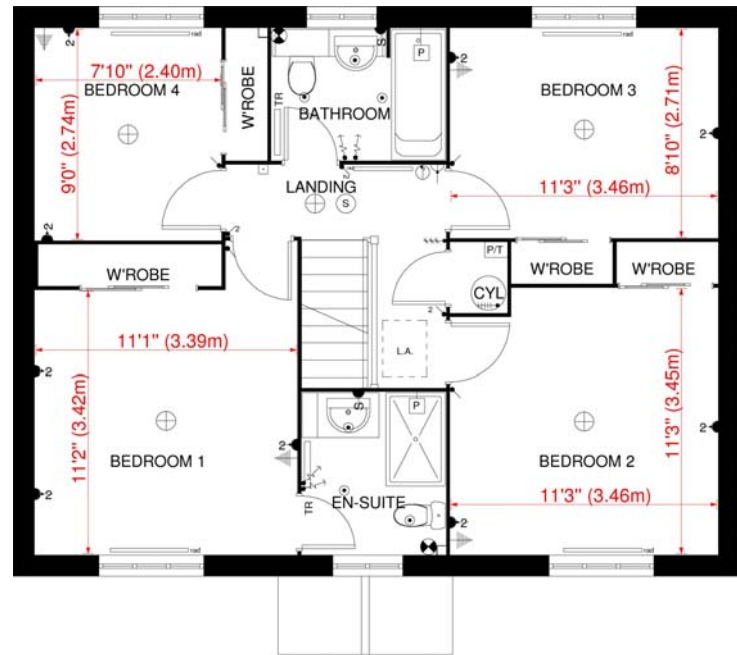
FIRST FLOOR PLAN 'ADDINGTON' HOUSE TYPE - BRADWELL
