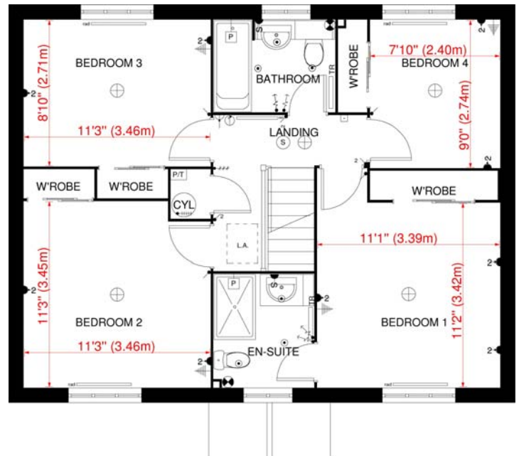
FIRST FLOOR PLAN (Handed) 'ADDINGTON 'B' HOUSE TYPE - BRADWELL
