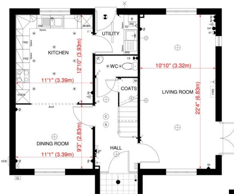
GROUND FLOOR PLAN (Handed) 'ADDINGTON 'B' HOUSE TYPE - BRADWELL
